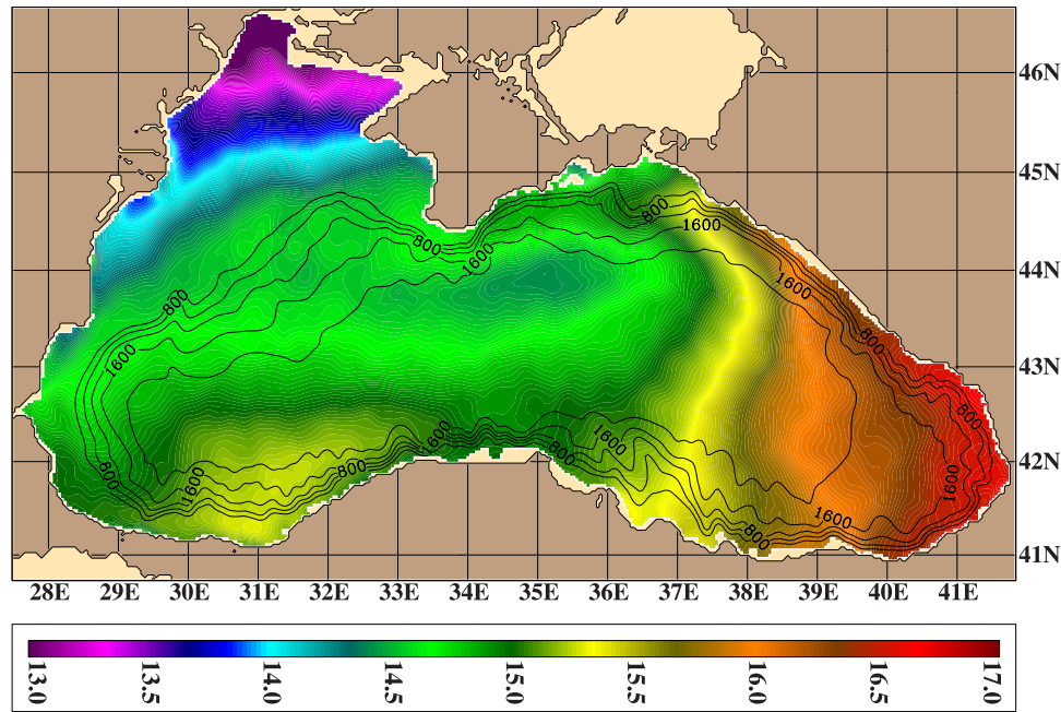
Figure 1. Climatological (annual) mean SST (°C) in the Black Sea. Bottom topography contours are also overlain, starting from 400 m with 400 m intervals.
