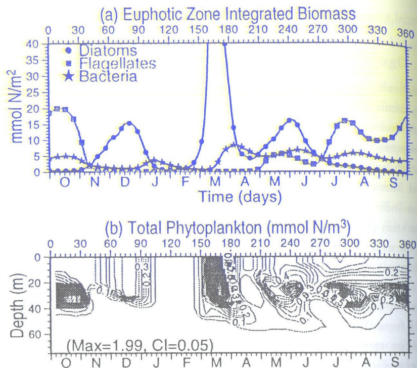
Figure 2. Annual distributions of the (a) euphotic zone integrated diatom, flagellate and bacterioplankton biomasses, (b) vertical structure of the total phytoplankton biomass within the upper layer water column computed by Oguz et al. (1998b)
