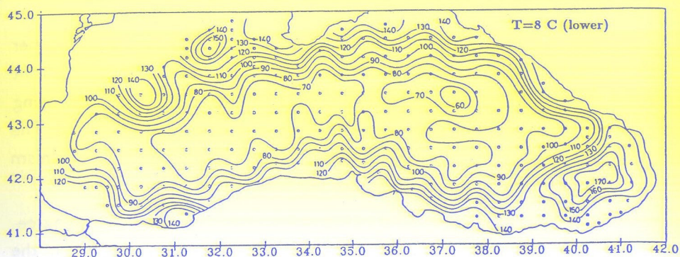
Figure 9a. Topography of the lower boundary of the Cold Intermediate Layer.
