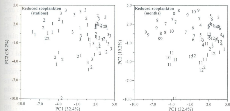
Fig. 6. PCA ordination of reduced zooplankton data. Projection of stations and months.
