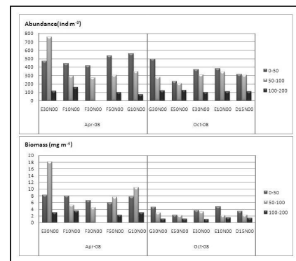
Fig. 2. Changes in mesozooplankton biomass and abundance in all sampling stations
