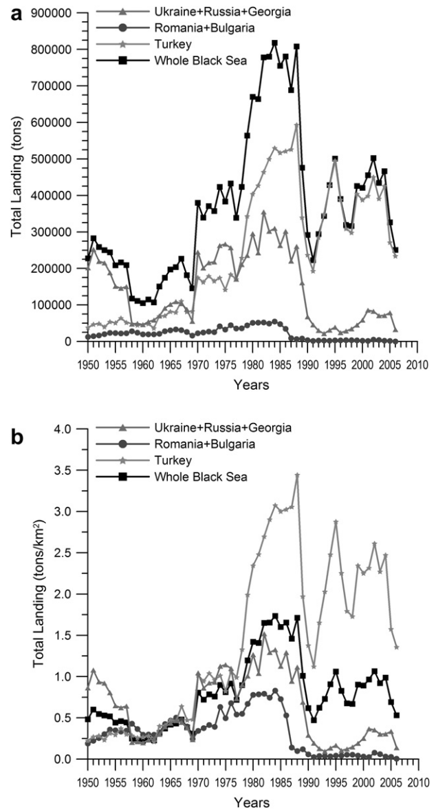
Fig. 4. Time series of (a) the total annual landings and (b) the annual landings per km^2 in the former USSR countries (Georgia + Russia + Ukraine), the western sector as the combination of Bulgaria and Romania, the southern sector of Turkish water, and over the whole Black Sea.
