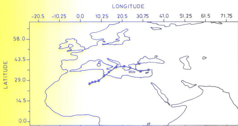
Figure 2. Air mass trajectory associated with sample 3-4 October 1991.
