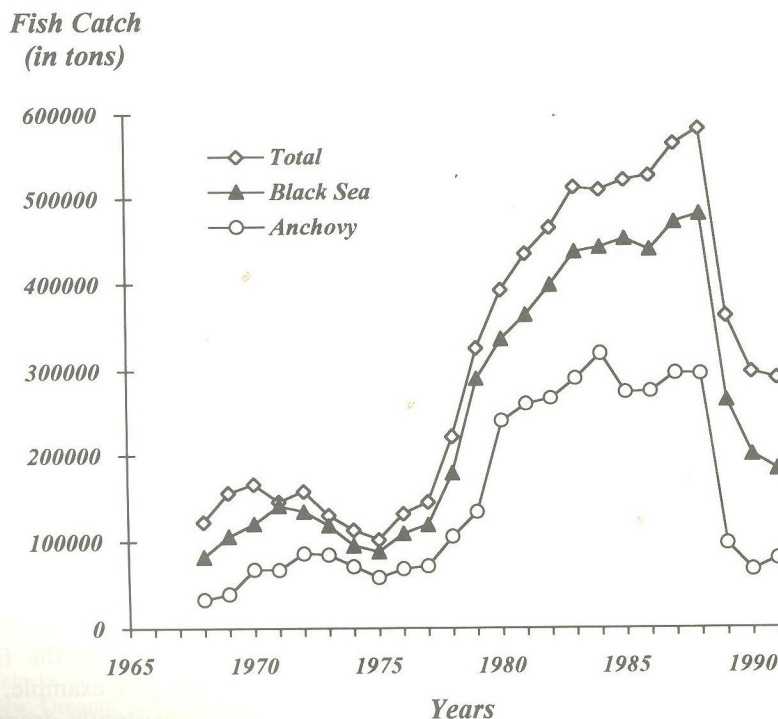
Fig. 1. Importance of anchovy fishing in the total Turkish catch between 1968 and 1991 (source SIS, 1968–1991).
