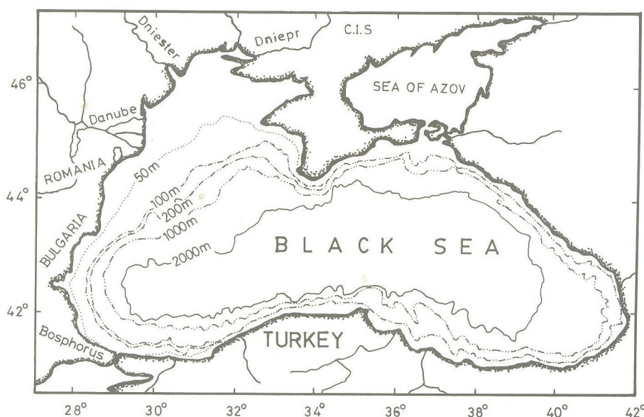
Fig. 2. The Black Sea (depth contours are labeled in meters).
