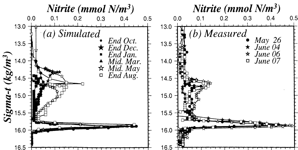
Figure 9. (a) The model simulated daily averaged nitrite profiles versus sigma- t ( \text{kg m}^{-3} ) at selected times of the year, (b) the observed nitrite profiles versus sigma- t ( \text{kg m}^{-3} ) obtained by the R/V Knorr surveys in the Black Sea during summer 1988. The concentrations are expressed in units of \text{mmol N m}^{-3} .
