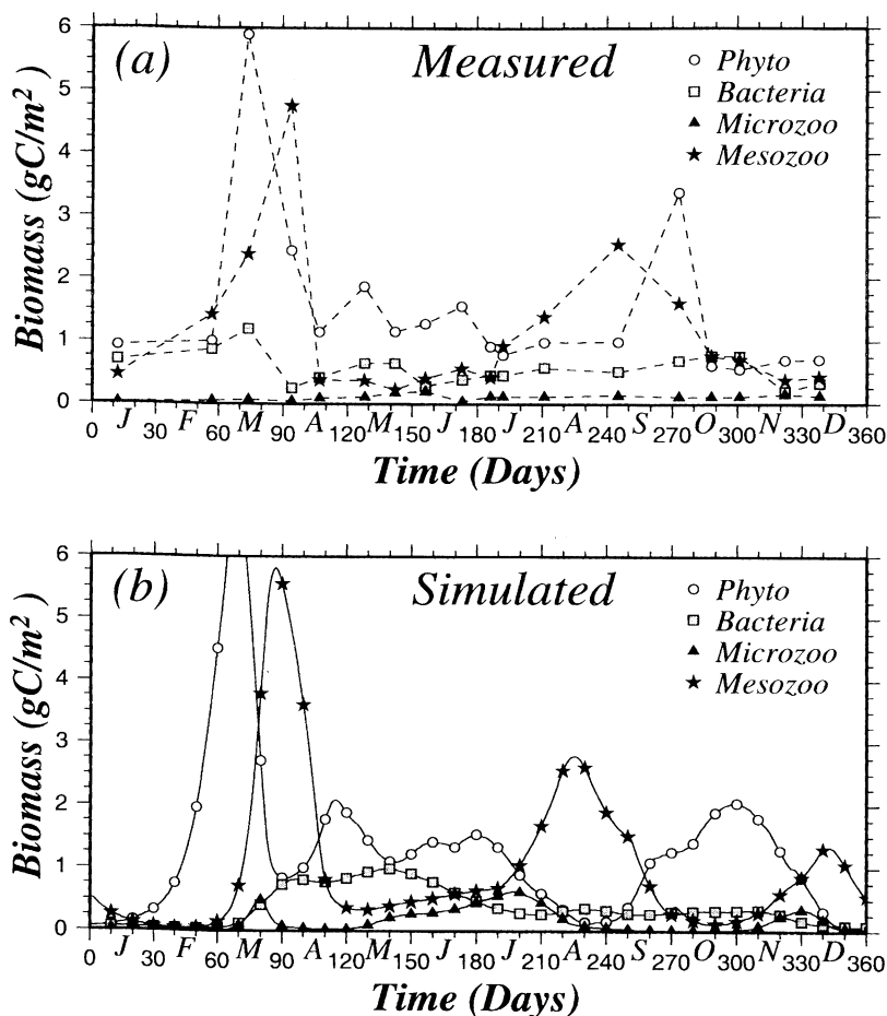
Figure 4. Temporal variations of water column integrated phytoplankton, bacterioplankton, microzooplankton, and mesozooplankton biomass (a) observed at a station off Gelendzhik during 1978 (after Shushkina et al. , [1983]) and (b) simulated by the model.
