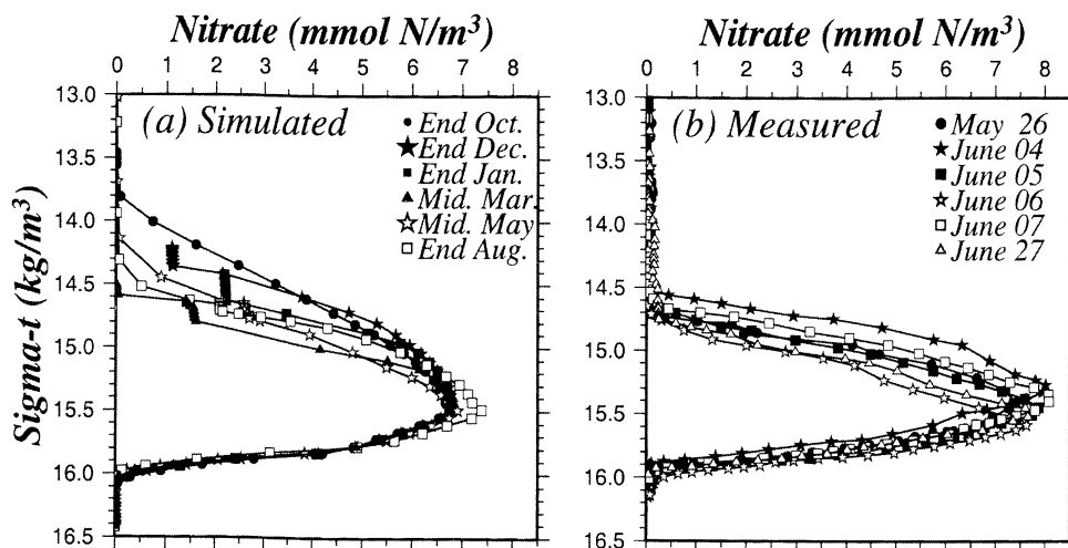
Figure 7. (a) The model simulated, and (b) observed nitrate profiles versus sigma-t ( \text{kg m}^{-3} ) at selected times of the year. The observed profiles were obtained by the R/V Knorr surveys in the Black Sea during summer 1988. The concentrations are expressed in units of \text{mmol N m}^{-3} .
