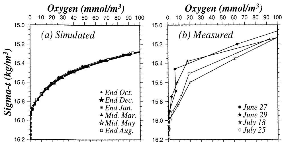
Figure 13. (a) The model simulated daily averaged dissolved oxygen profiles versus sigma-t (kg m -3 ) within the oxycline and suboxic layers of the water column at selected times of the year, (b) the observed dissolved oxygen profiles versus sigma-t obtained by the R/V Knorr surveys in the Black Sea during summer 1988.
