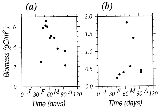
Figure 12. Observed (a) phytoplankton and (b) mesozooplankton biomass distributions (in \text{gC m}^{-2} ) during February-April 1991. Each data value represents an average of several measurements within the interior basin.
