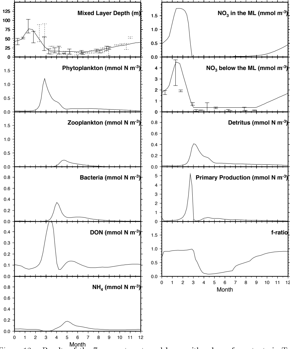
Figure 13. Results of the 7-compartment model run with values of constants in Table 1 for region 2. Bars show 95% confidence limits: solid bars, Bilim, HydroBlack and CoMSBlack cruises (1986-1995); dashed bars, Mamayev data (1926-1992).
