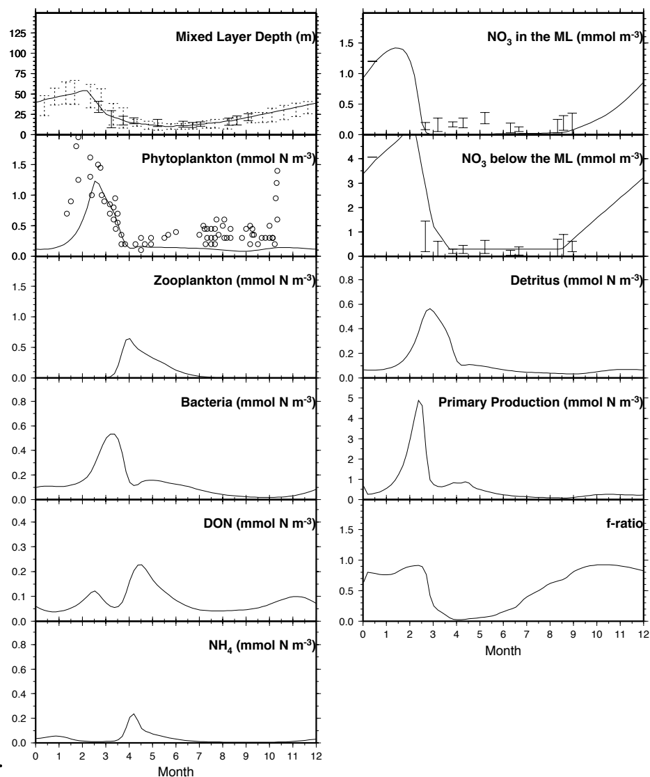
Figure 8. Results of the 7-compartment model run with values of constants in Table 1 for region 1. Open circles show the euphotic layer average chlorophyll concentrations mg\ Chl\ m^{-3} . The data are redrawn from Vedernikov and Demidov (1993).
