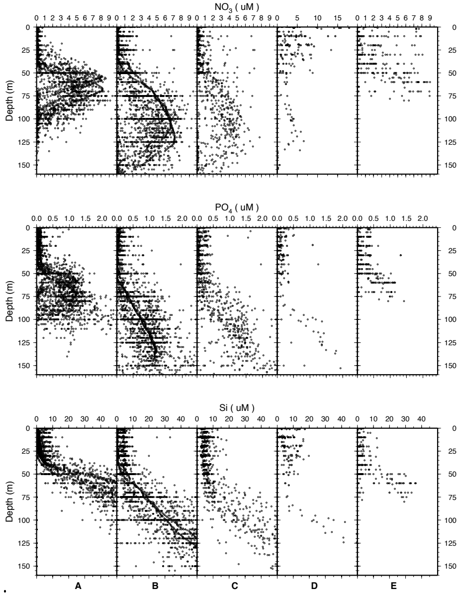
Figure 5. Variations of NO_3 , PO_4 and Si concentrations ( \mu M ) with respect to depth in the (A) cyclonic region, (B) anticyclonic regions (C) northwestern region, (D) the Danube estuary mouth region, (E) Bosphorus exit region.
