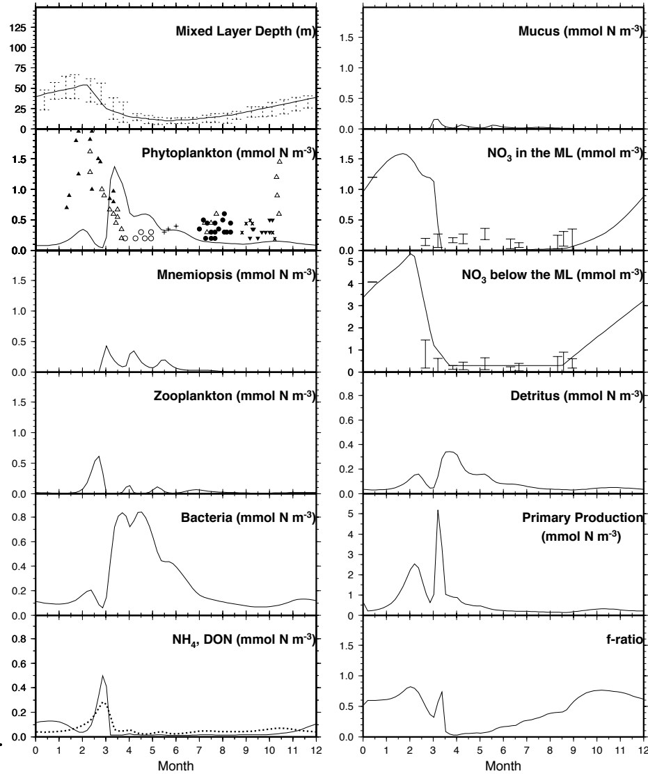
Figure 10. Results of model including Mnemiopsis , run with values of constants in Table 4 for region 1.
