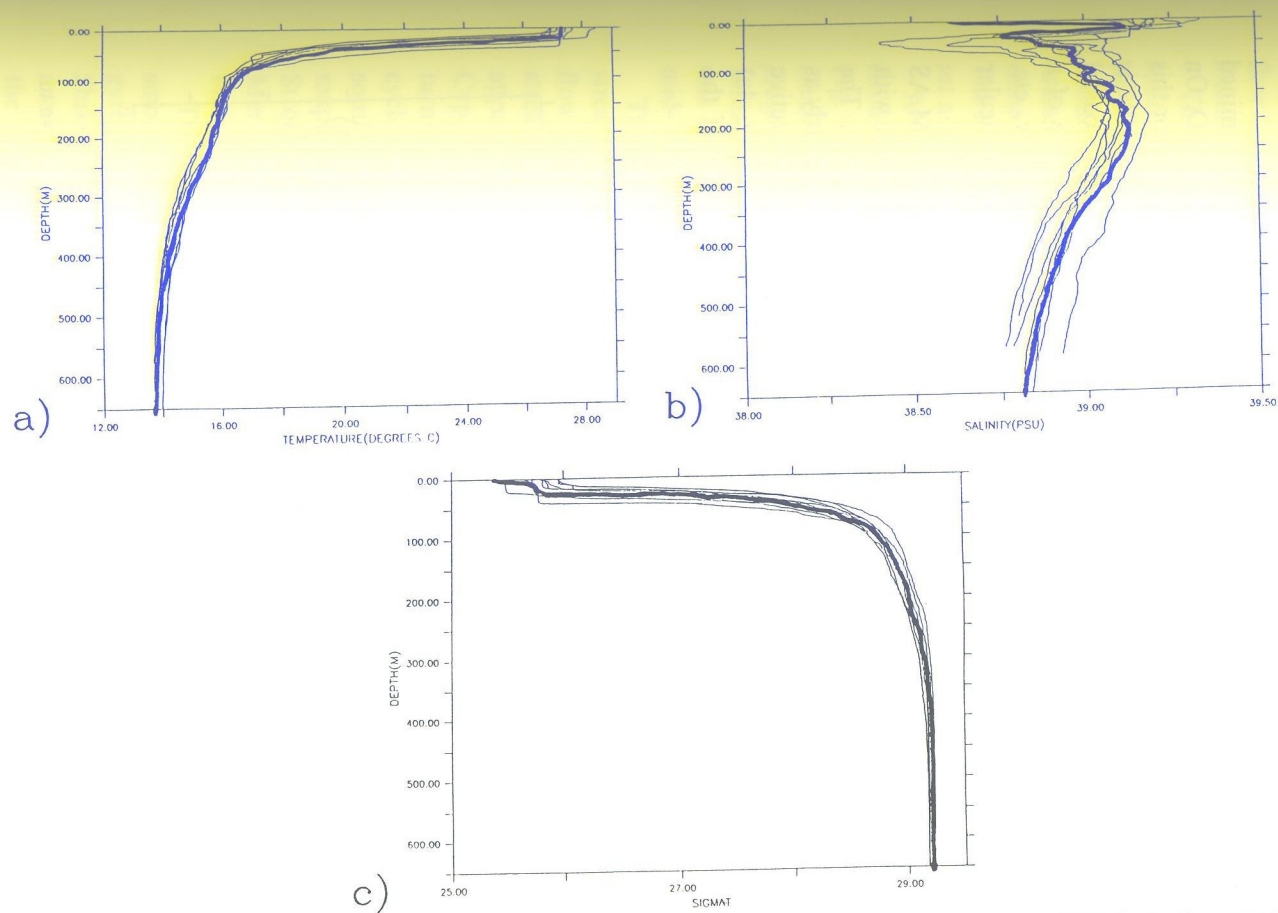
Fig. 5. Profiles of: (a) temperature; (b) salinity; (c) density ( \sigma_t ), for the stations near the northern Levantine coastal region with the selected boundary profile identified by the darker line.
