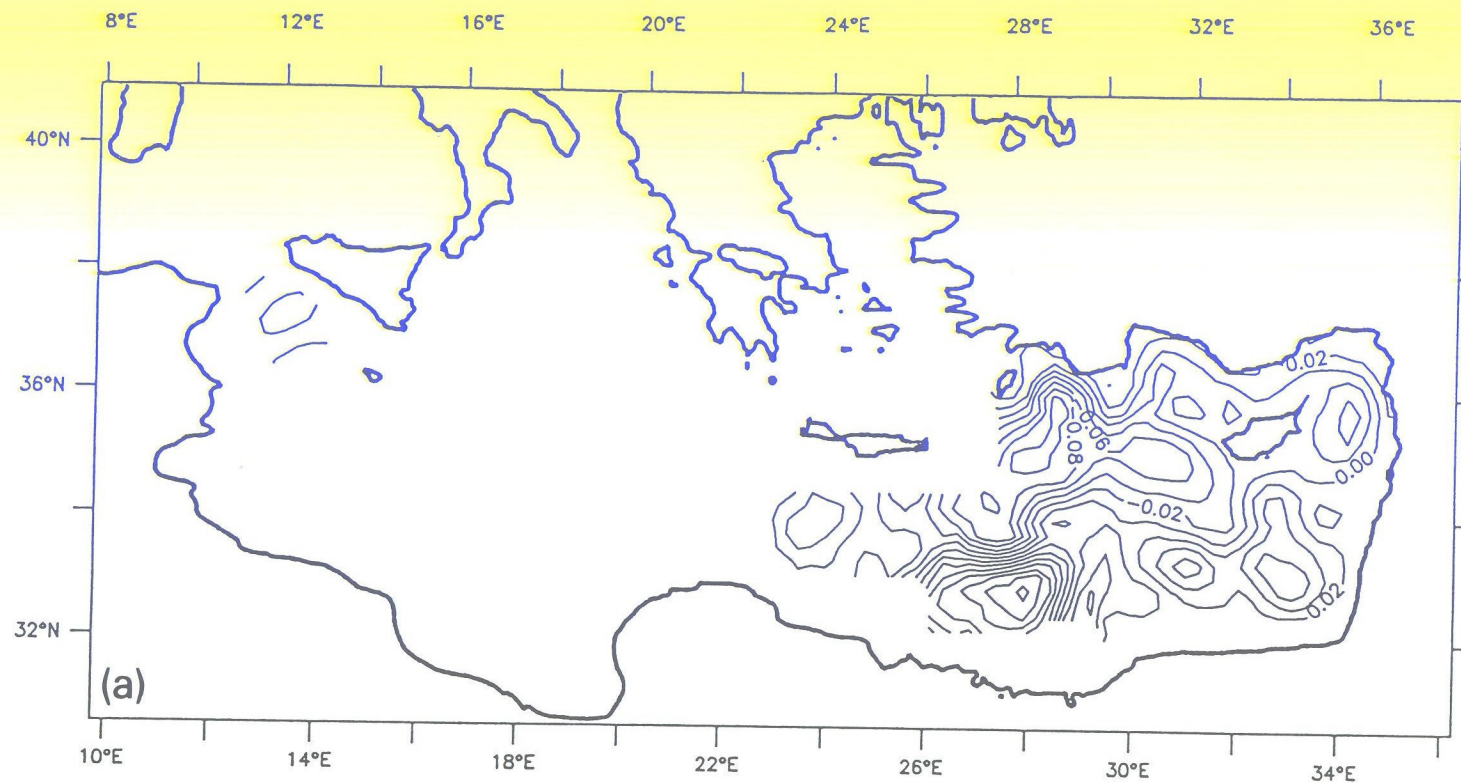
Fig. 8. As in Fig. 7 but for ON 85.
