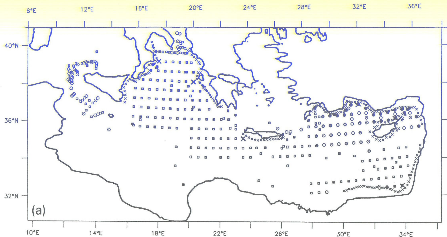
Fig. 3. Station locations indicated by ○ (deeper than 450 m and shallower than 800 m) and □ (deeper than 800 m), near-coastal profiles used in the selection of the boundary profile ● or ■, the selected profile coastal constraint × or ■, and the positions of inserted boundary profiles ×. (a) AS 87, (b) ON 85, (c) MA 86, (d) MA 87.
