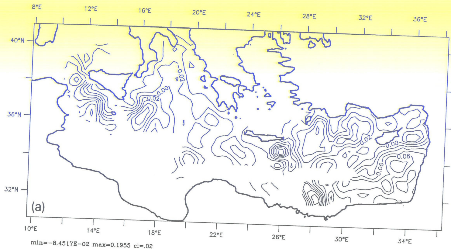
Fig. 7. (a) Dynamic height anomaly (dm), upper thermocline (30/450) with coastal constraint, AS 87. (b) Horizontal flow vectors at 30 m, AS 87.
