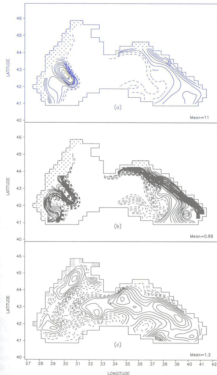
Figure 11. Snapshots of 3-D numerical model simulations at 19 March, 1982 for (a) depths of isopycnal surface \sigma_t=14.4 , CI=5 m; (b) Nitrates concentrations at isopycnal surface \sigma_t=14.4 , CI=0.1 mmol N m -3 ; (c) Nitrates concentrations at depth 17.5 m, CI=0.1 mmol N m -3 .
