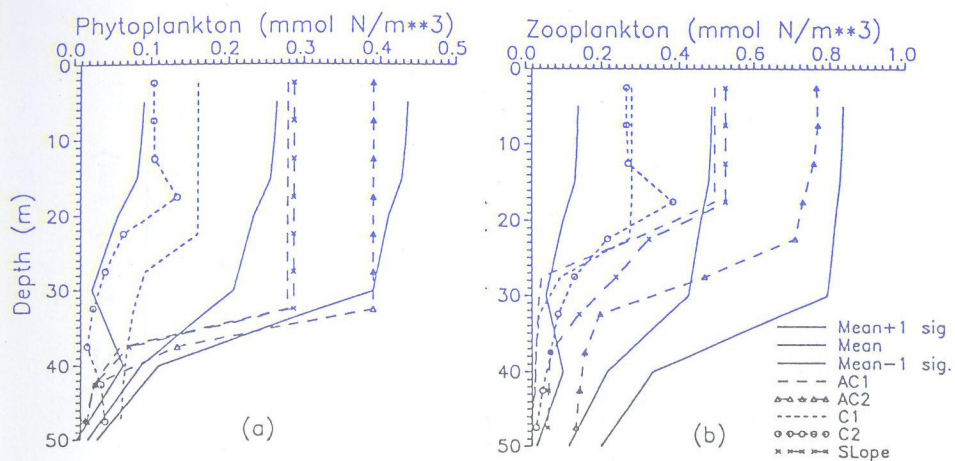
Figure 10. Vertical profiles at 12 April 1986. Simulations from the one dimensional physical/biological mixed layer model in the five sample locations are plotted with dash lines. Area averaged and 1-\sigma deviations from the area averaged simulated in 3-D OGCM are plotted with full lines. (a) phytoplankton; (b) zooplankton.
