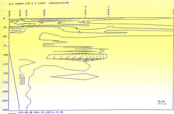
Figure 9. Distribution of light transmission (%) along transect B, including stations 2,3,5,6,7,8,9.
