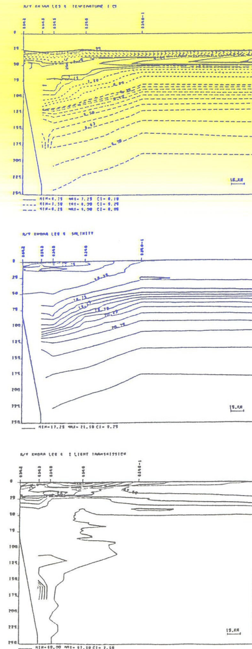
Figure 8. Distribution of (a) temperature ( ^{\circ}\text{C} ), (b) salinity, and (c) light transmission (%) along transect A, including stations 2,3,5,6,8,9.
