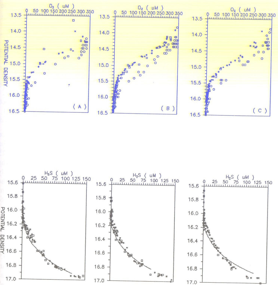
Figure 3. Potential density dependent variations of dissolved oxygen and hydrogen sulfide within dynamically different regions of the Black Sea. (A): cyclonic, (B): anticyclonic and (C): rim current for Bilim-91 (*) Knorr-88 (—), Prof. Kolesnikov-91 (□) and Atlantis-69 (○) data.
