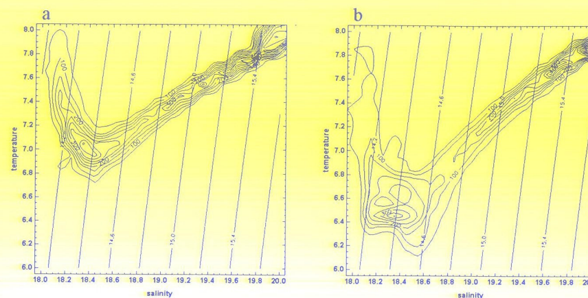
Figure 3 a,b. Volumetric T,S diagrams ( \text{km}^3 per 0.1^\circ\text{C} , 0.1 \text{ T,S class} ) for August-91 (a) & July-92 (b).
