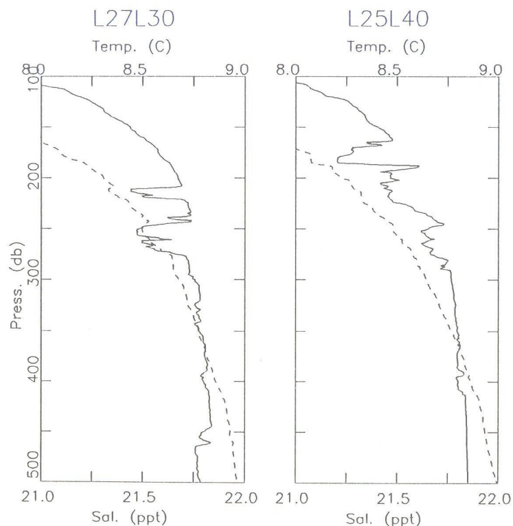
Figure 9. Temperature and salinity profiles during April 1989 at two stations L27L30 ( 41^{\circ} 27'N and 29^{\circ} 30'E ) and L25L40 ( 41^{\circ} 25'N and 29^{\circ} 40'E ) located near the shelf break adjacent to station L25L15. See the location map in Figure 10 for positions of stations
